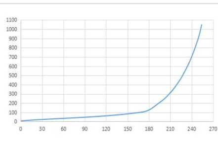
DALI Dimming Curve (logarithmic)
